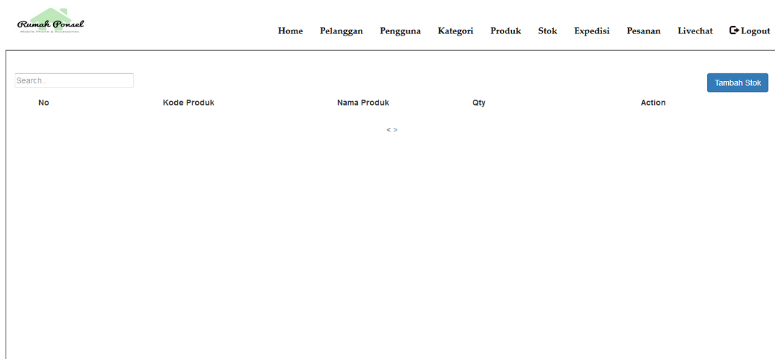
Gambar 5.11 Halaman Stok
