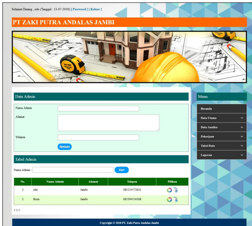
Gambar 5.2 Data Admin
