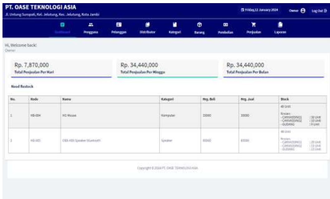
Gambar 5.1 Halaman Dashboard
