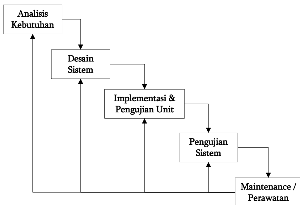
Gambar 3.2 Model Waterfall [38]
