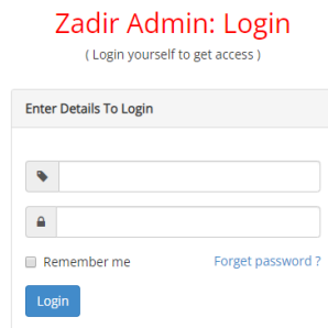
Gambar 5.7 Login Admin
