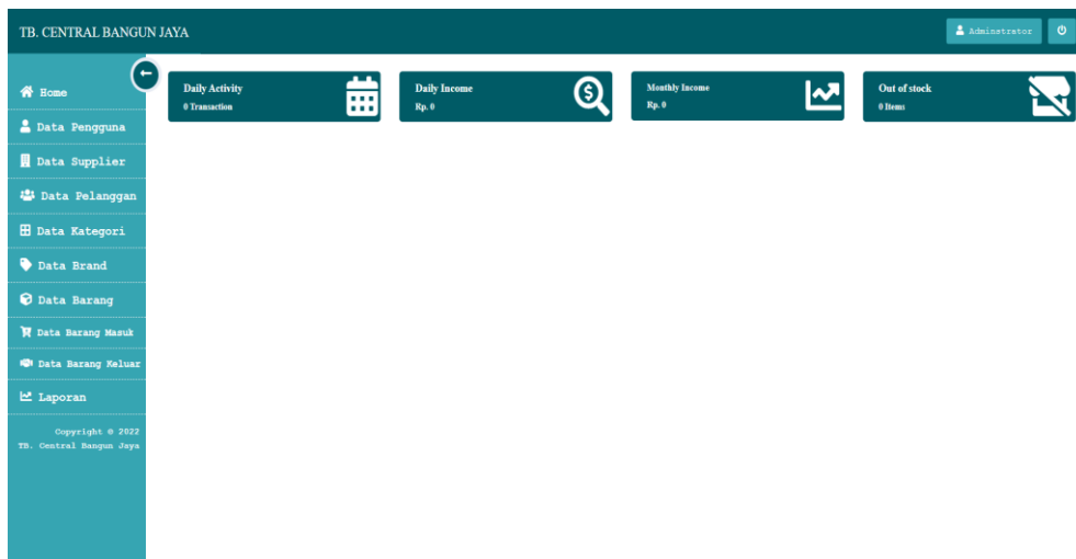
Gambar 5.1 Halaman Home
