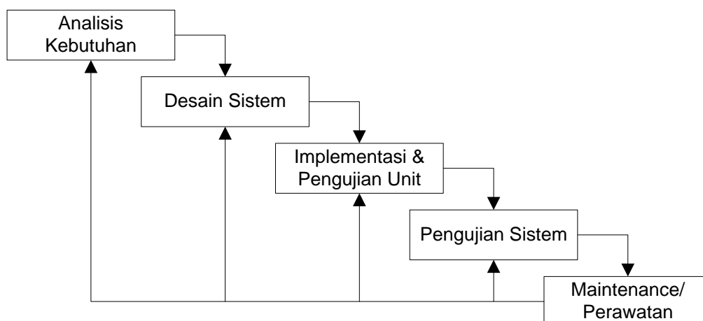
Gambar 3.2 Model Waterfall [44]
