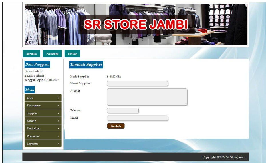
Gambar 5.5 Tambah Supplier
