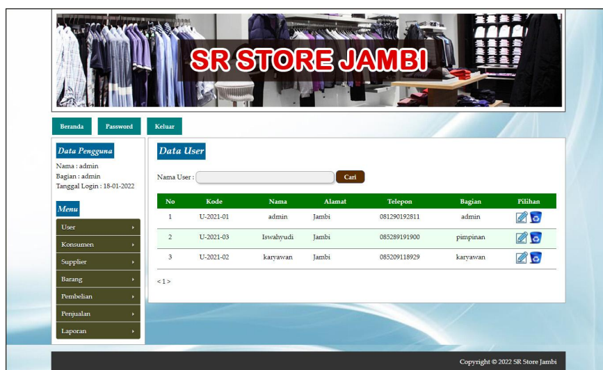
Gambar 5.3 Tambah User
