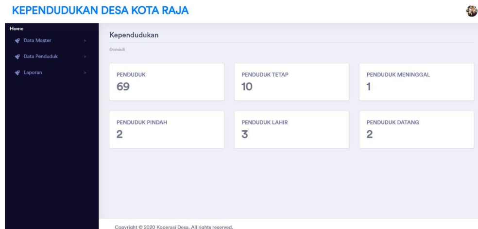
Gambar 5.21 Tampilan Dashboard
