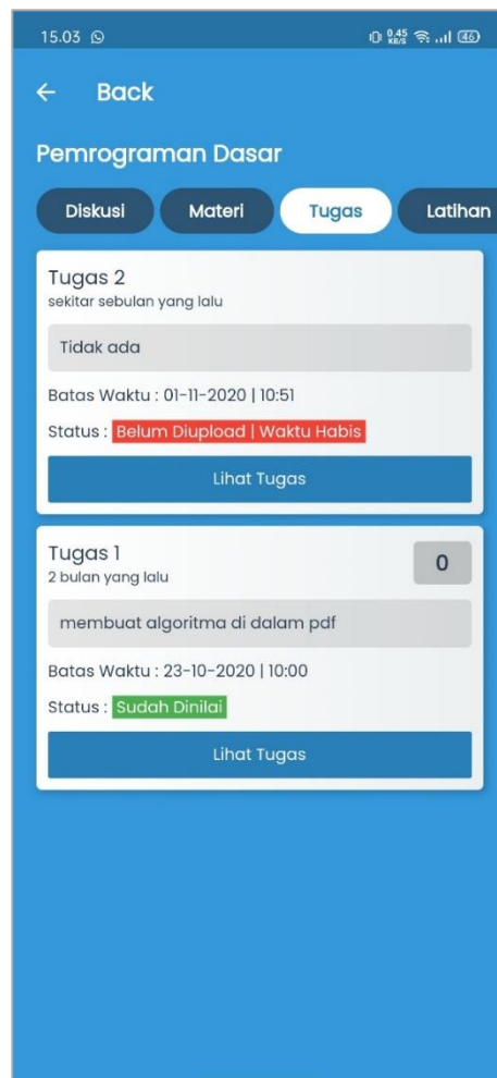
Gambar 5.26 Halaman Tugas
