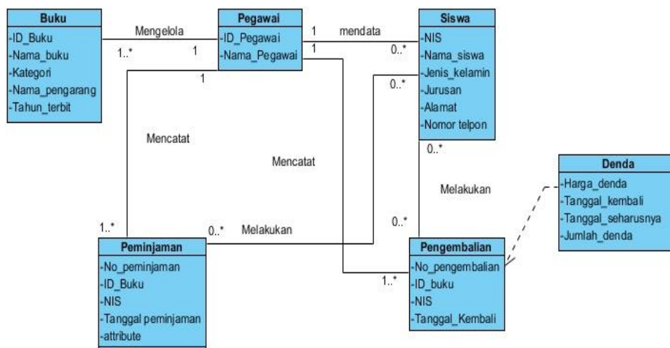
Gambar 5.6 Class diagram Perpustakaan
