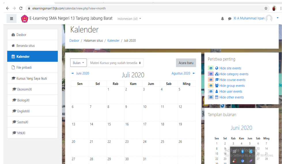
Gambar 5.14 Halaman Kalender
