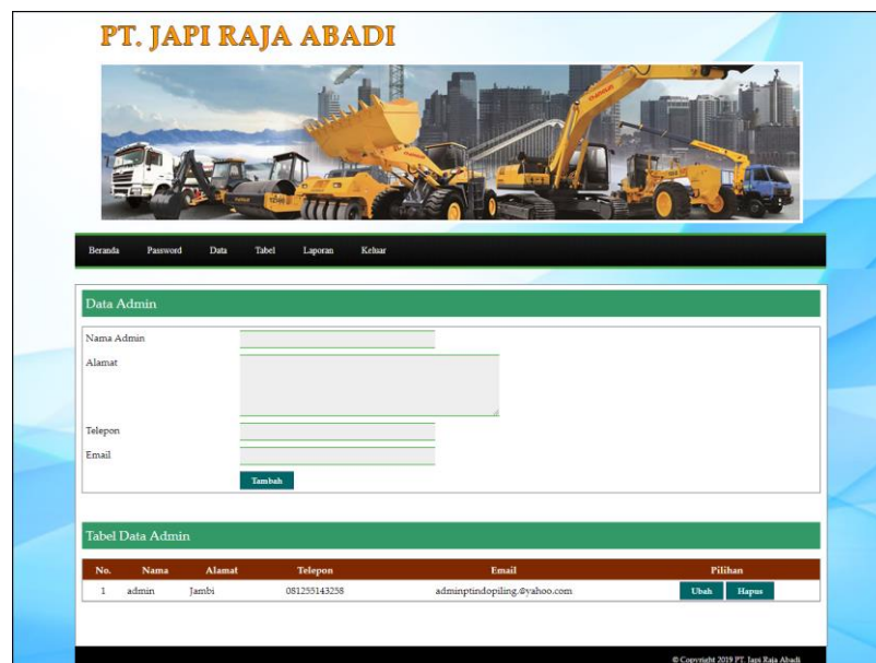
Gambar 5.8 Data Admin
