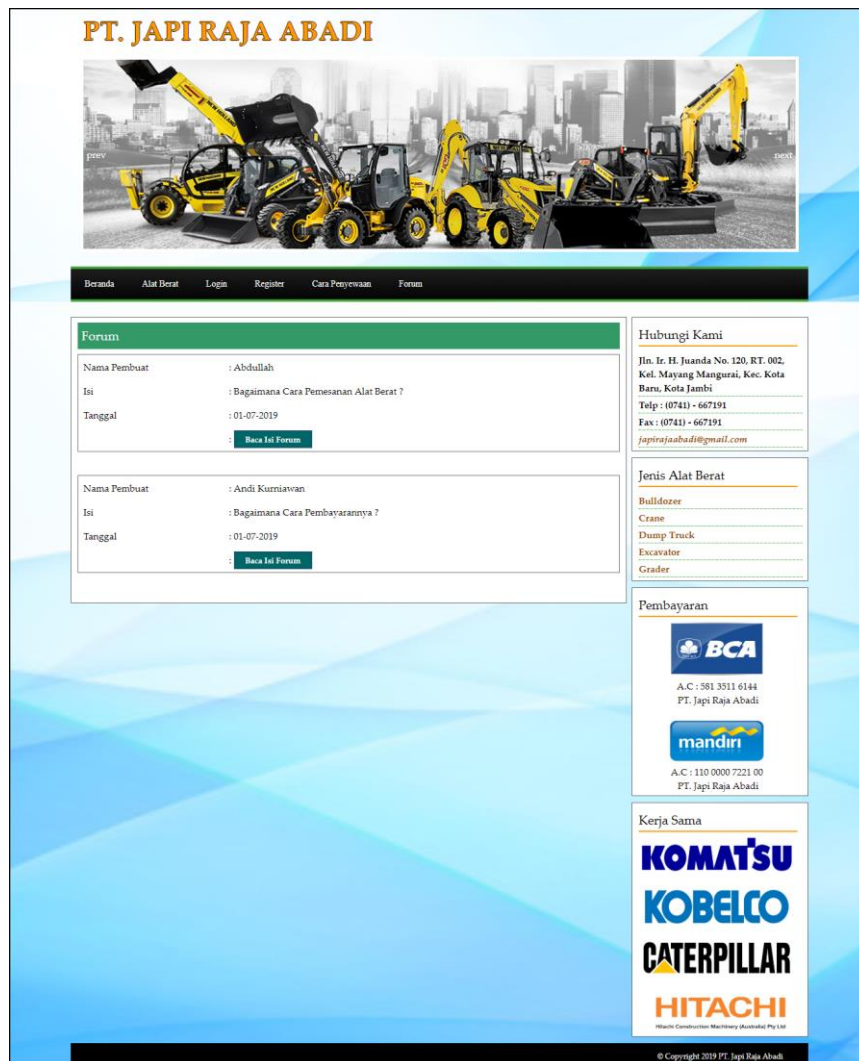
Gambar 5.13 Tabel Forum
